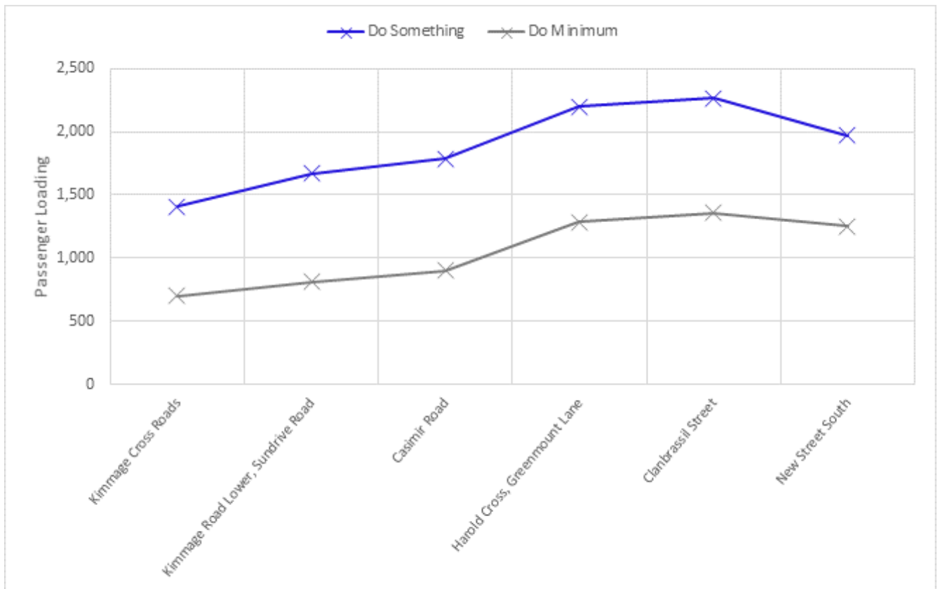
Image 2.11: 2028 AM Peak Hour Passenger Volume Along Proposed Scheme (Inbound Direction)
